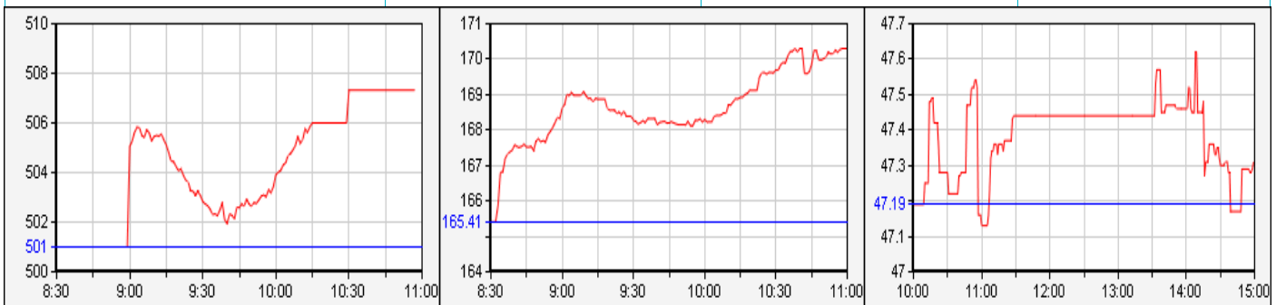
VN-INDEX
